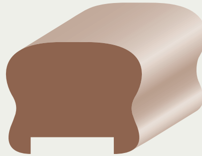
926P 1-1/2 x 1-7/8 Doug Fir Handrail plowed 1/4 x 1-1/4
