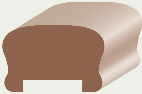
925P 1-1/2 x 2-3/8 Doug Fir Handrail plowed 1/4 x 1-1/4
