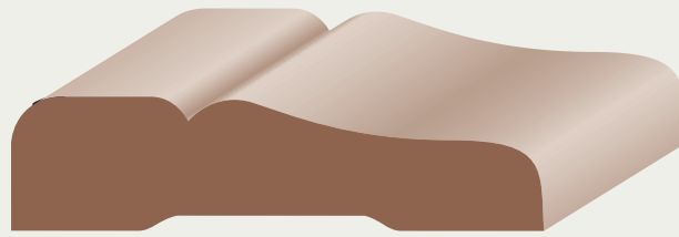
108VG 5/8 x 2-1/2 VGDF 711 Casing
